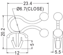
CHASSIS Ø4.0 THICKNESS 1.6-4.0
