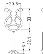
CHASSIS Ø4.8-Ø5.0 THICKNESS 0.5-2.3
