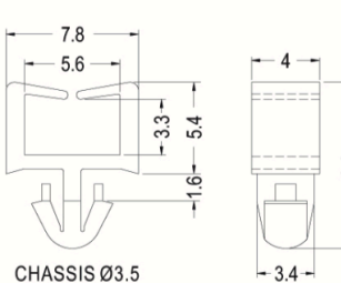
CHASSIS Ø3.5 THICKNESS 1.5
