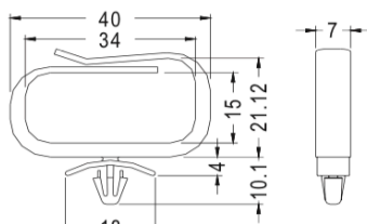
CHASSIS Ø4.8 THICKNESS 0.8~2.0
