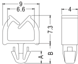
CHASSIS Ø3.5
