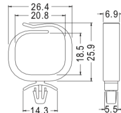
CHASSIS Ø4.8~Ø5.0 THICKNESS 0.8~2.0
