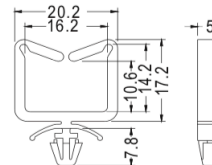
CHASSIS Ø4.8 THICKNESS 1.0-2.5
