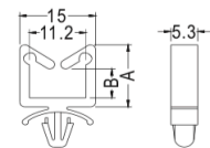
CHASSIS Ø4.8-Ø5.0 THICKNESS 0.8-2.0
