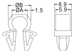
CHASSIS Ø6.0 THICKNESS 2.0
