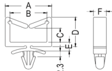
CHASSIS Ø4.8-Ø5.0 THICKNESS 1.2-2.1
