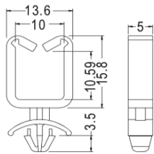
CHASSIS Ø5 THICKNESS 0.8~1.6
