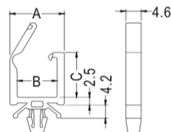
CHASSIS Ø4.8 THICKNESS 0.5~2.0
