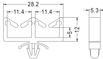
CHASSIS Ø4.8~Ø5.0 THICKNESS 1.2~2.1
