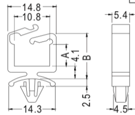
CHASSIS Ø4.8~Ø5.0 THICKNESS 0.5~2.0
