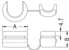
CHASSIS Ø19 THICKNESS 0.8~1.6
